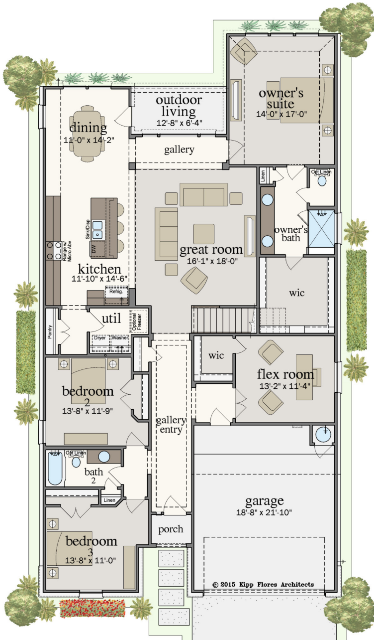
FIRST FLOOR
