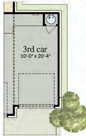
OPTIONAL 3RD CAR GARAGE
