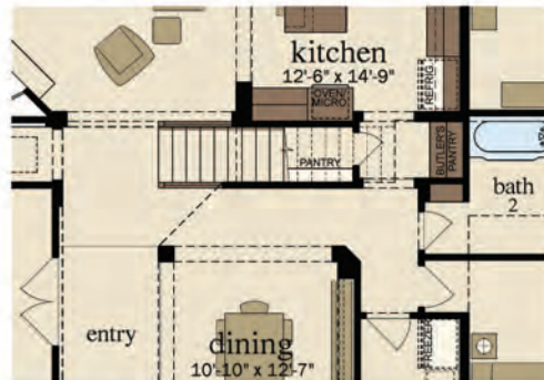
FIRST FLOOR STAIRS W/ OPTIONAL SECOND FLOOR
